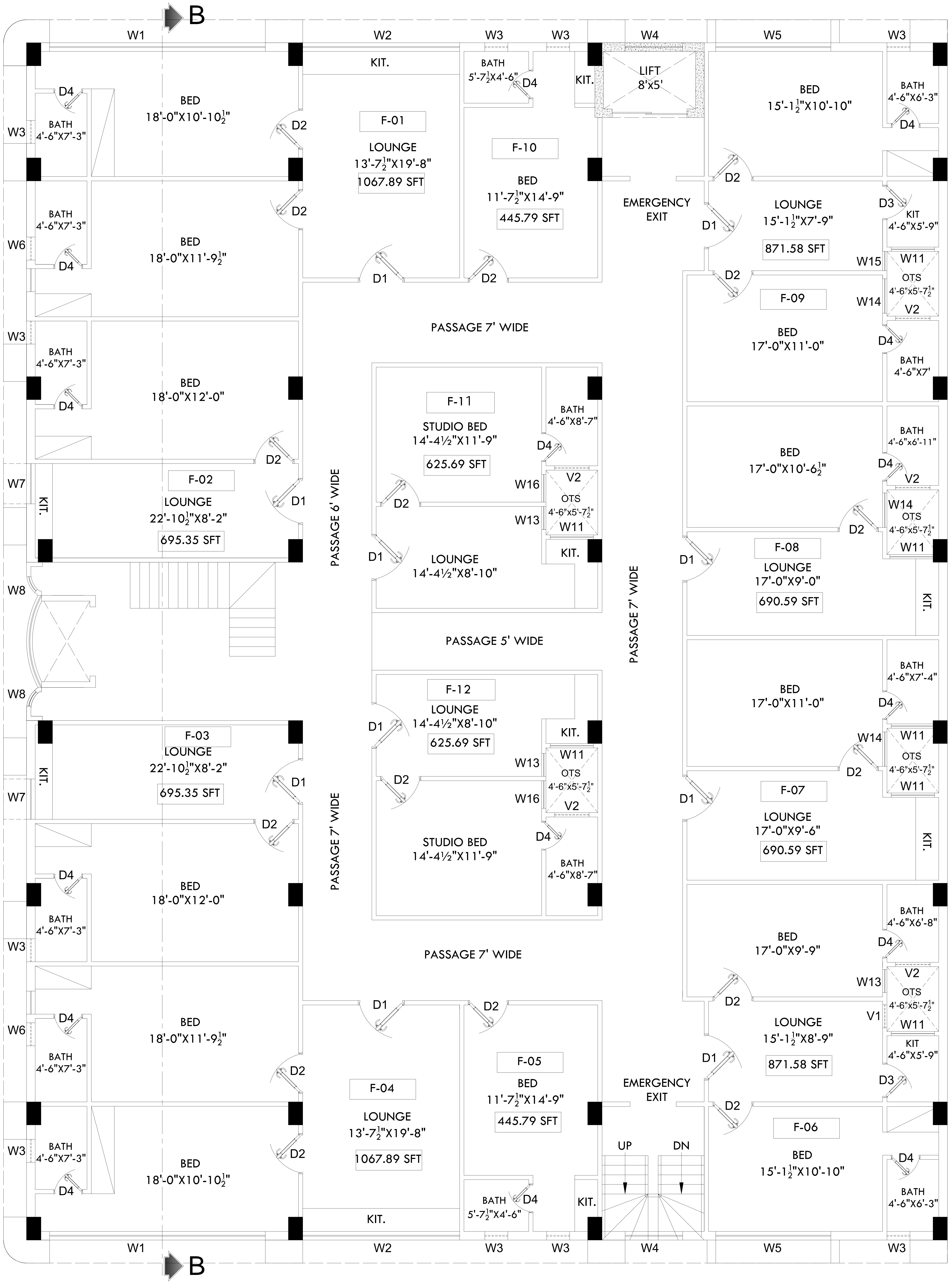
FOURTH FLOOR PLAN/ TWO BEDS
